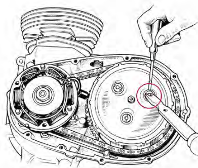
Fig. C5. Unscrewing the clutch spring nuts
