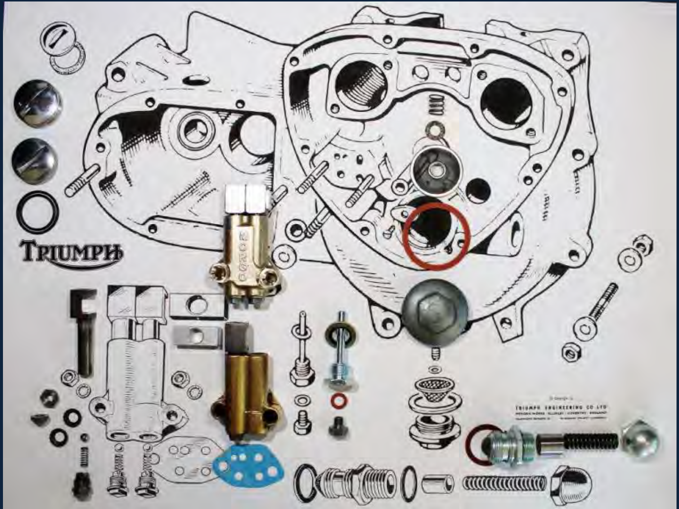
The Oil Pump, Relief Valve, Sump Filter and Gearbox Drain and Level Plug.
