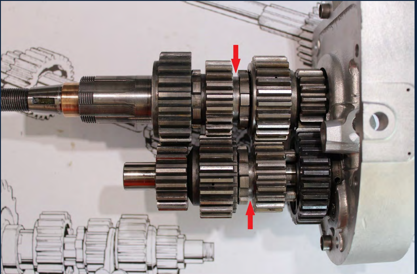
Gear Clusters Assembled onto the Intermediate Cover.
