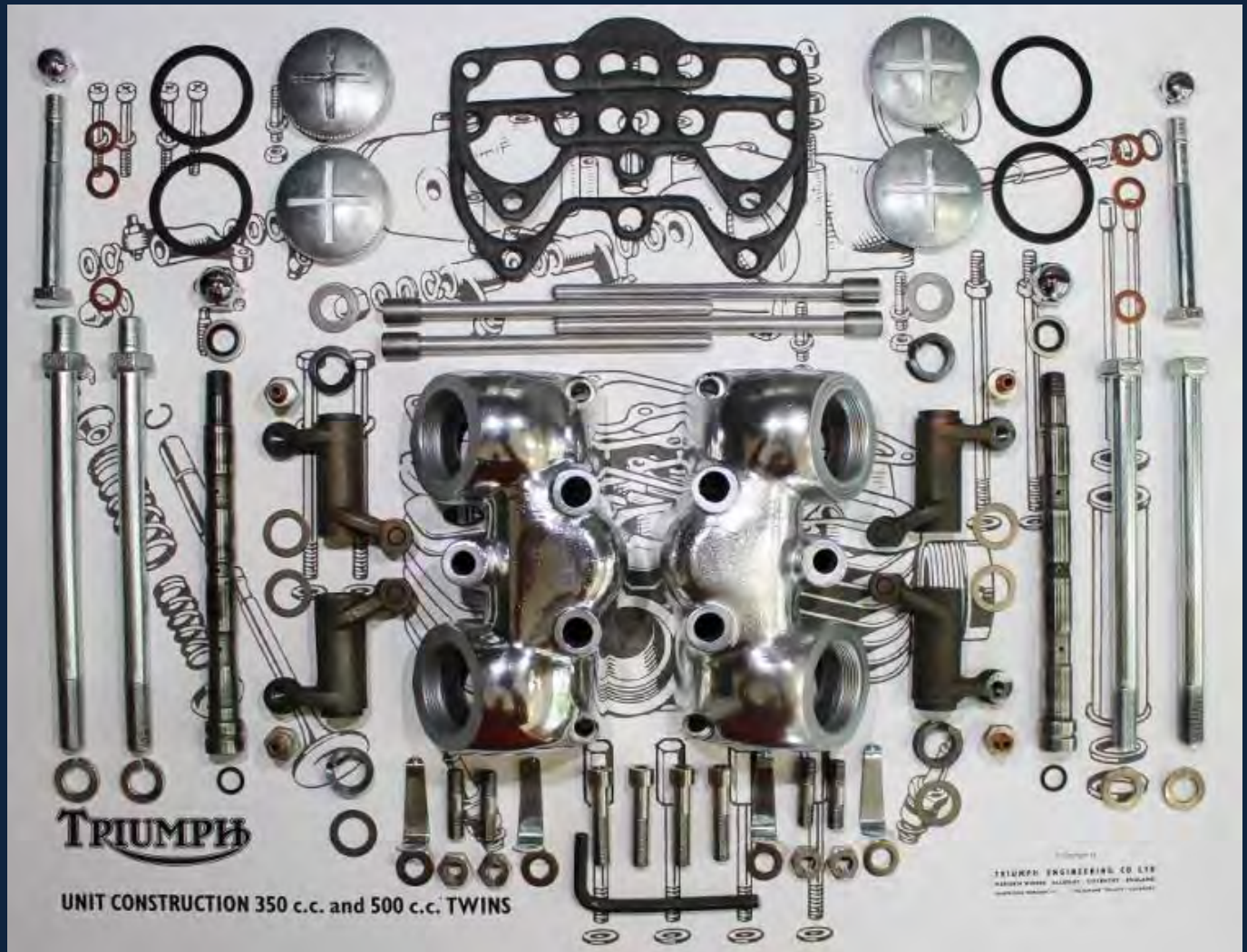
The Rocker Boxes and Parts.
