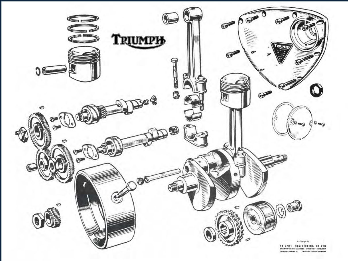
One of the Images from the Triumph Parts Book
