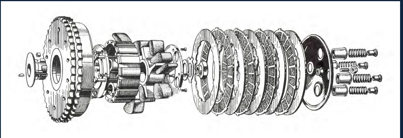
The 1957 to 1963 Four Spring Clutch
