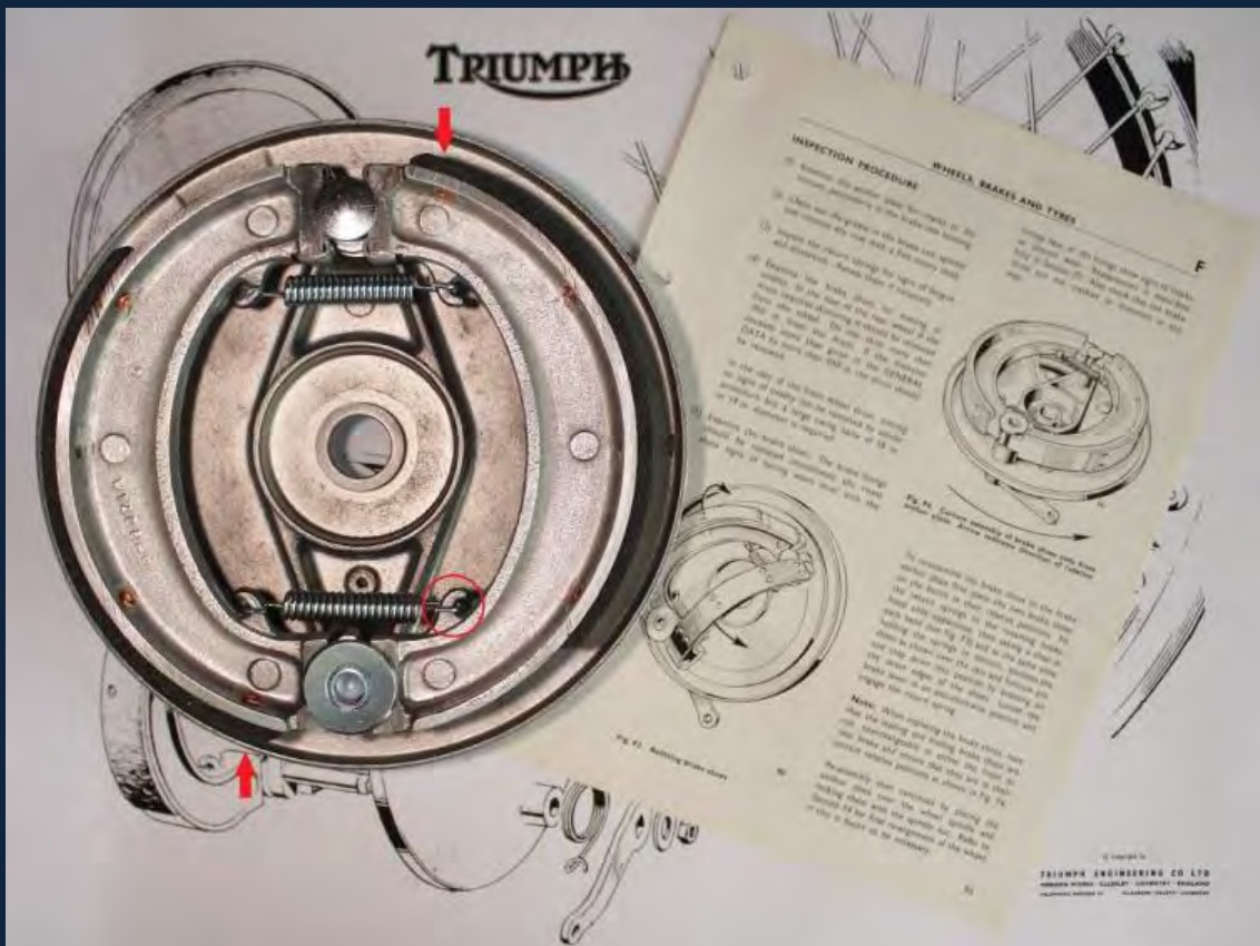
The Correctly Assembled Brake
