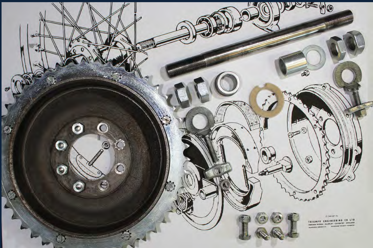
The Standard drum (non QD) and the arrangement of the axle, parts and fasteners.
