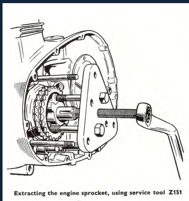
Showing the service tool Z151, for removing the drive sprockets and separating the crankcases, this handy tool is relatively easy to make with CAD, (Cardboard Aided Design)
