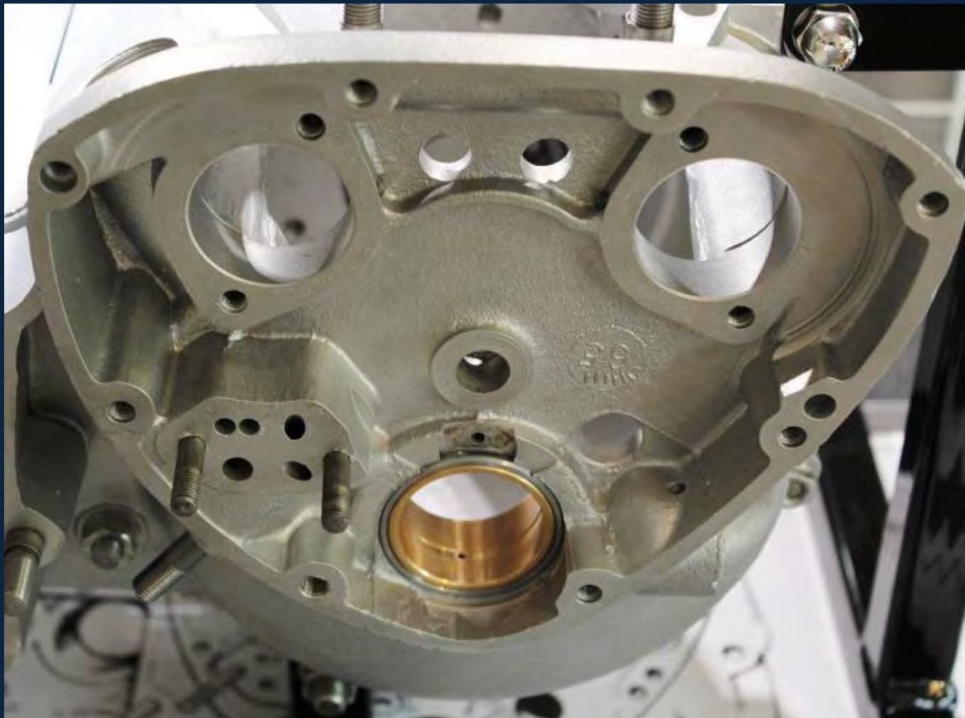
The Timing Side Bush Fitted
