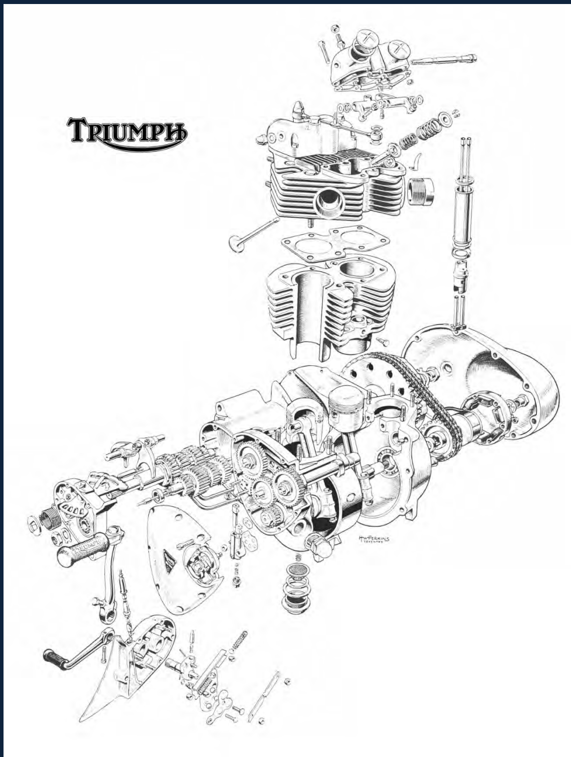
The Engine Cutaway Drawing (1963 onwards)
