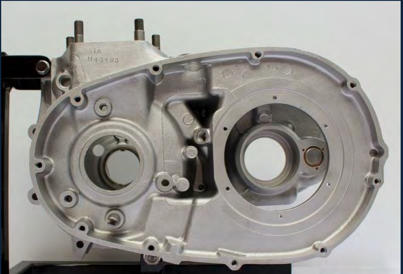
Crankcase Left Side.
