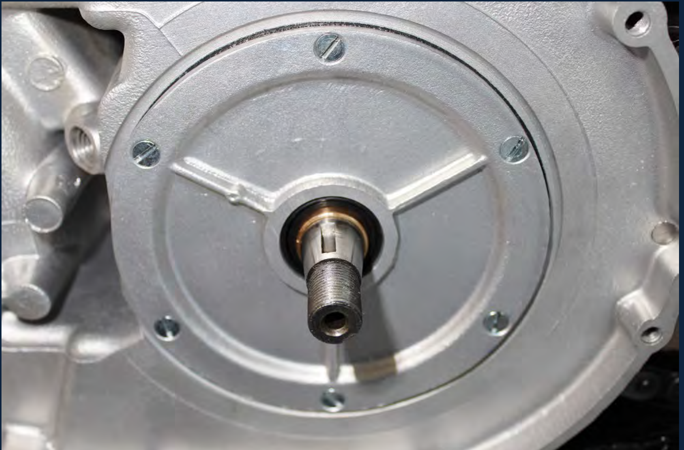
The 1966 Access Plate and the blanked off chain Oil Feed Quill
