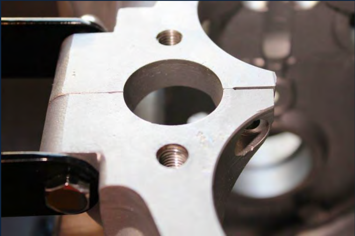
Two of the Eight Cylinder Stud Holes 3/8 BSF.
