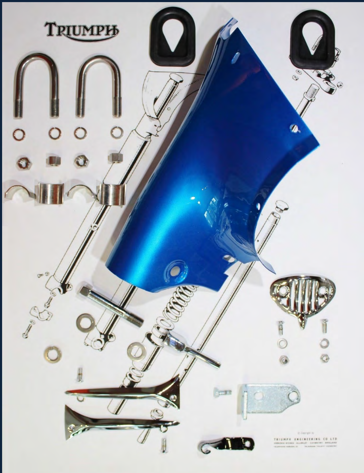
Some of the parts of the Nacelle for the 1966 3TA
