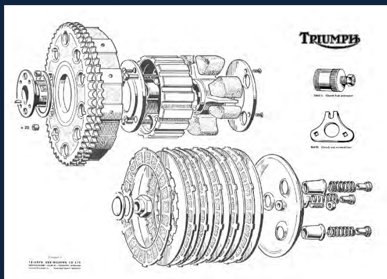
The General Arrangement of the Triumph Clutch
