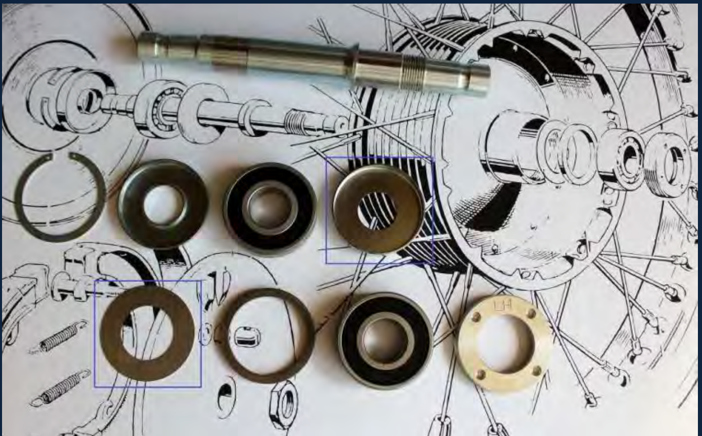
Front Wheel Axle and Bearing Set. Section F of the Works Manual
