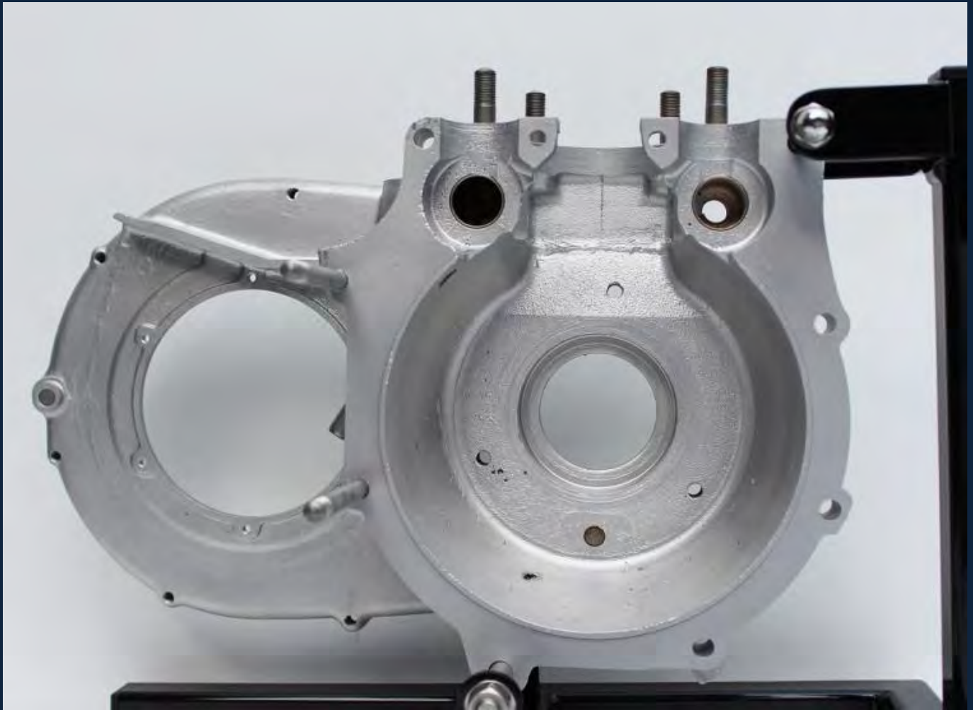
Crankcase Drive Side Internal View.
