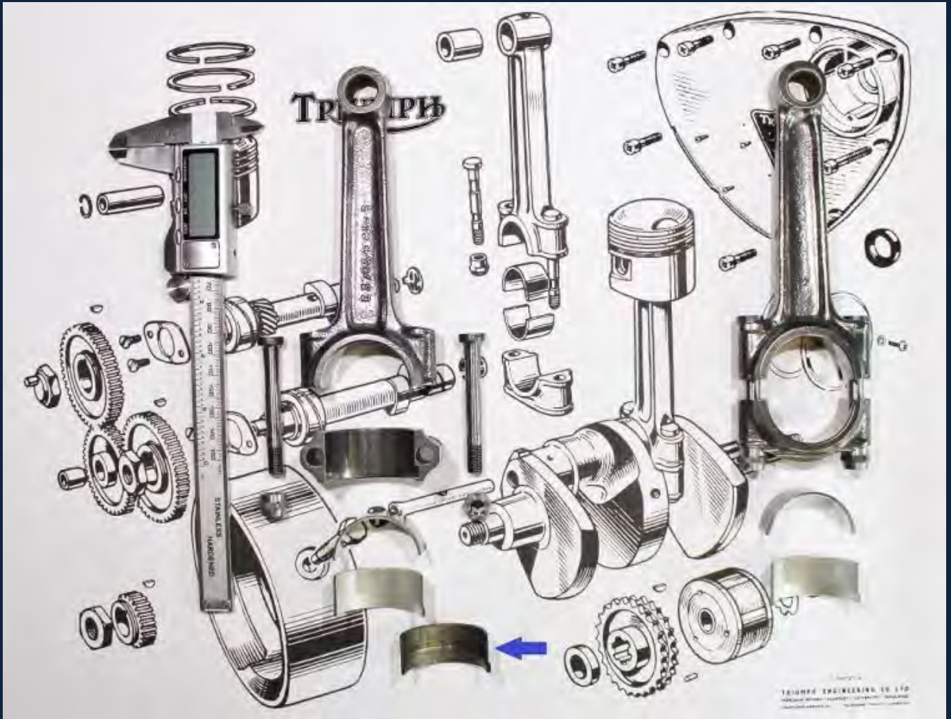
The Connecting Rods, Caps, Shell Bearings and Bolts.
