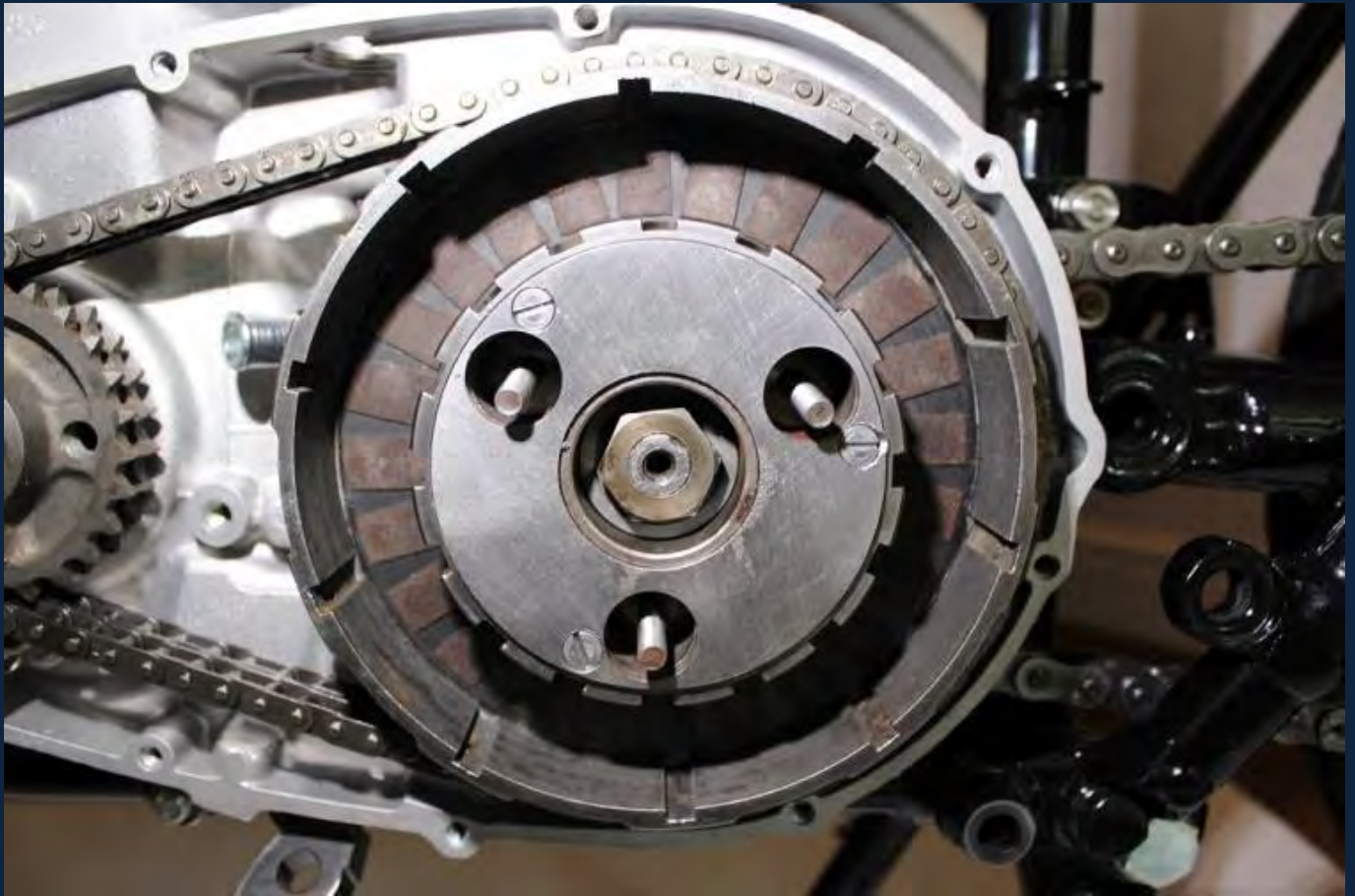
Shock Absorber and 1 st Driving Plate Fitted
